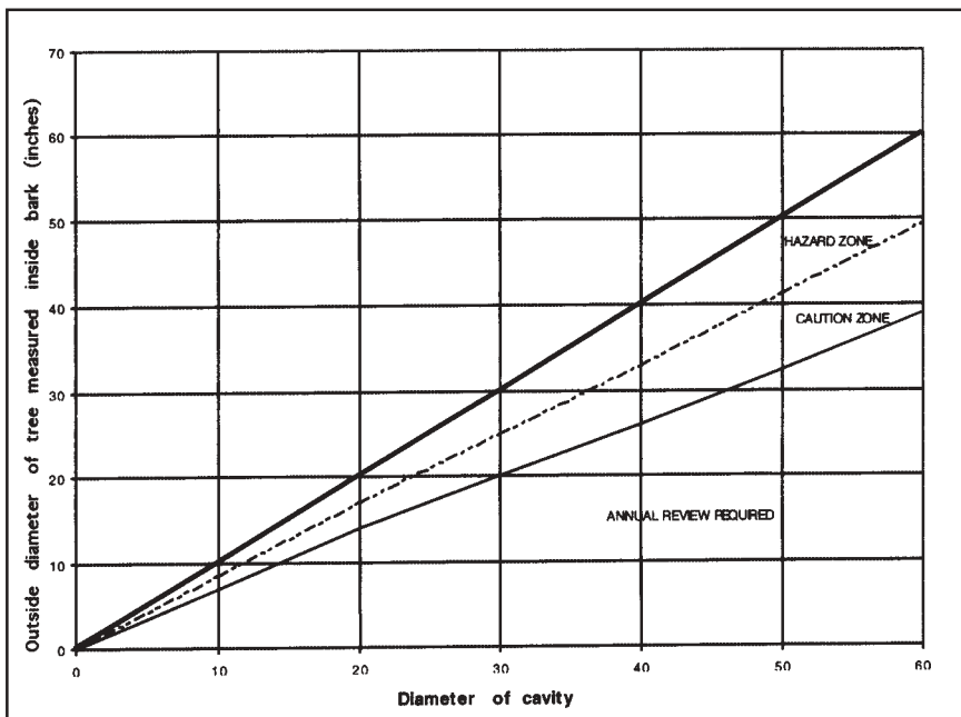
Figure 4. Strength loss graph to accompany Coder's d^4 \div D^4 formula. Trees having lost 20% to 44% of their strength due to decay are in the caution zone; when strength loss rises above 44%, the tree should be considered hazardous (Coder 1989).
