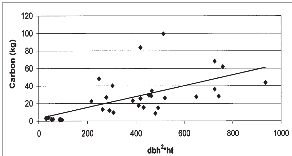
Figure 4. Carbon stored by Malus cultivars. Allometric regression equation is y = 0.0217x^{1.1574} ; R^2 = 0.7425 or 74%.
