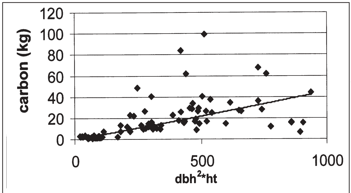
Figure 2. Carbon stored in Amelanchier, Pyrus calleryana, Malus, and Syringa reticulata cultivars according to dbh 2 * ht. Allometric regression equation is y = 0.0272x^{1.0718} , R^2 = 0.707 or 71%.
