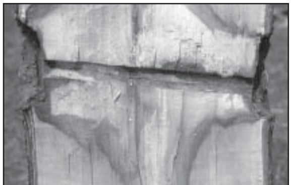
Figure 2. Some years after installation of a crown anchor: The bolt with a diameter of 18 mm (0.7 in.) led to discoloration and white rot above and below the drill hole.
