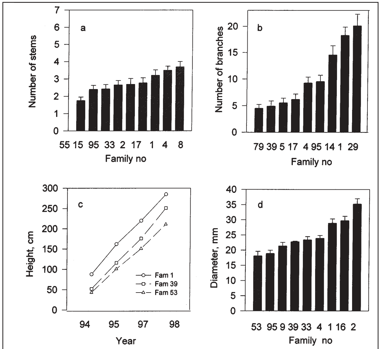
Figure 2. Number of stems (a), number of branches (b), tree height (c), and diameter of the main stem (d) in some rowan families. The values are means \pm standard error, n = 28–30.
