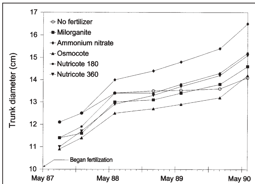
Figure 2. Trunk diameter for 3 years after transplanting live oak receiving 5 different sources of nitrogen fertilizer.
