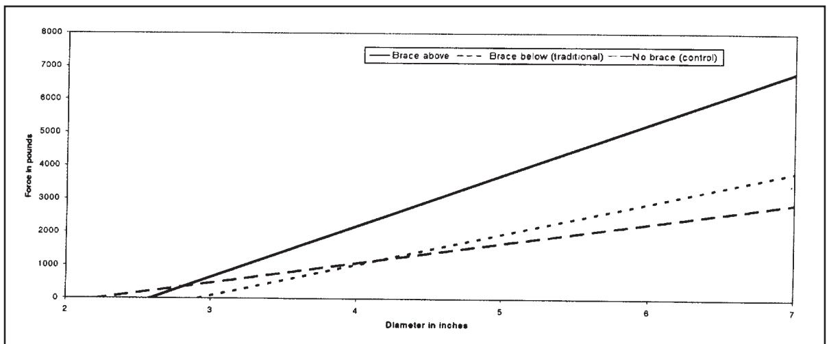
Figure 6. Comparison of breaking strengths on red oak crotch systems with no bracing (control), traditional rod placement at the crotch, and rod located above the crotch.
