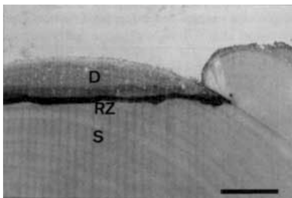
Figure 1. Reaction zone behind a wound that has destroyed the bark of a sycamore ( Acer pseudo-platanus ) tree. A green reaction zone [RZ] has formed between the decaying, exposed wood [D], and the healthy, underlying sapwood [S]. Scale bar = 20 mm (0.8 in.)
