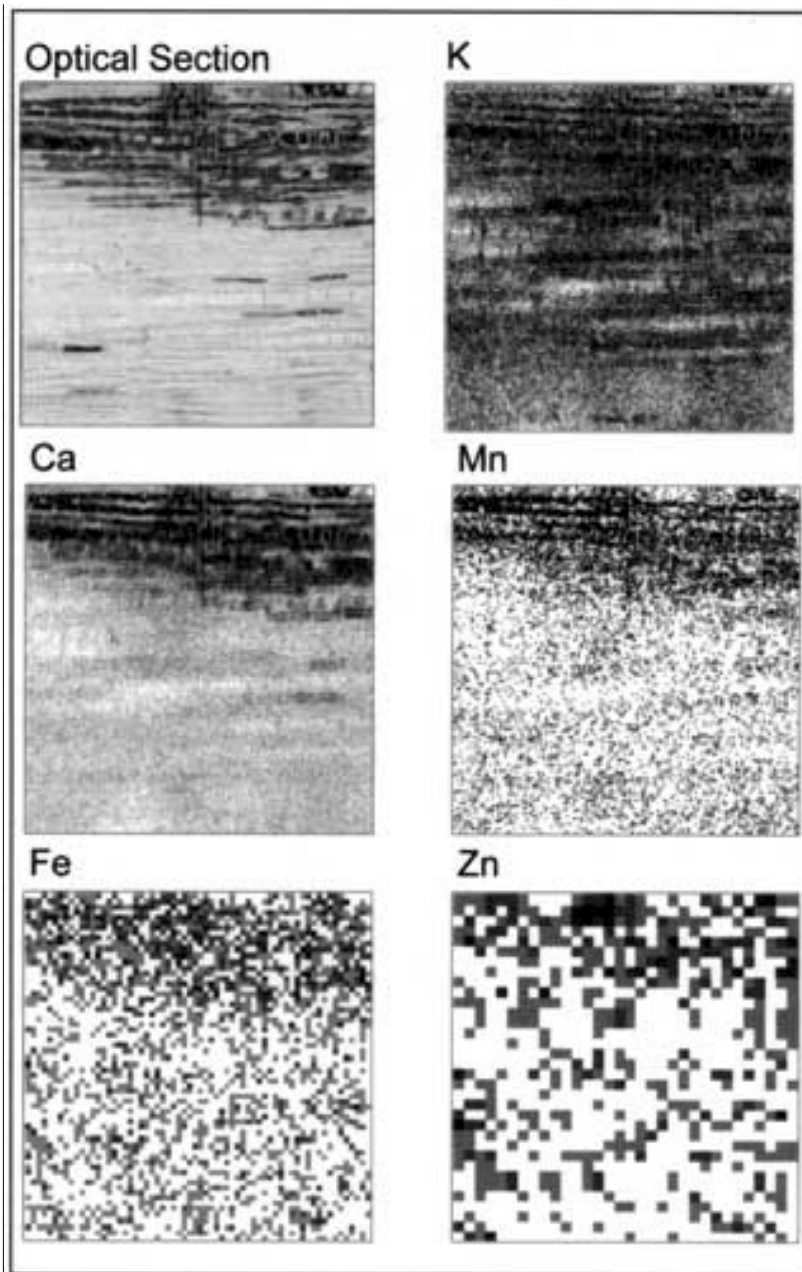
Figure 6. Elemental distribution in a reaction zone in beech ( Fagus sylvatica ), formed in the branch collar region at the base of a small branch that had died naturally. Elements were mapped using PIXE, essentially as described by Kramer et al. (1997), from a radial longitudinal section (15 \mu\text{m} thick) that included a fully developed reaction zone characterised by insoluble, brown, polymeric deposits, an intermediate region in which reaction zone responses were not fully developed, and healthy wood (see optical section). PIXE maps of potassium (K), calcium (Ca), manganese (Mn), iron (Fe), and zinc (Zn) show the accumulation of these elements in the discolored reaction zone. Potassium concentrations are also elevated in the intermediate tissues. Field = 750 \mu\text{m} .
