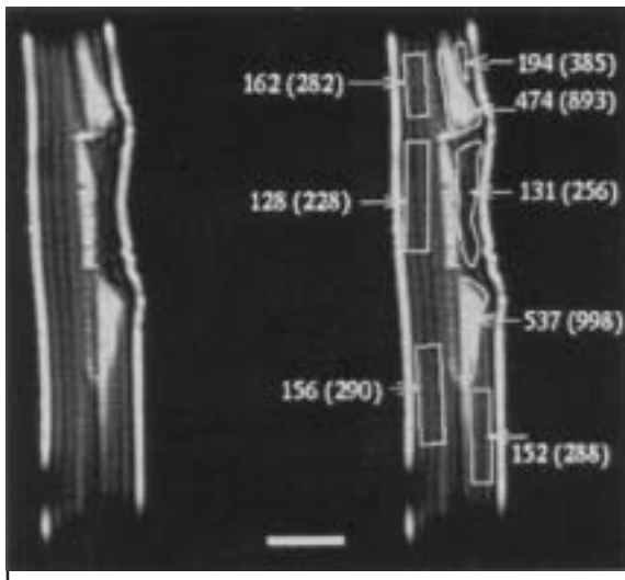
Figure 4. Spin-echo NMR image of a radial longitudinal slice through a juvenile sycamore stem 17 months after wounding and inoculation with the weakly aggressive decay fungus Ganoderma adspersum . Experimental details and full explanation are given in Pearce et al. (1997a). High-contrast cones of reaction zone tissue extend above (474) and below (537) the wound (131), which has become occluded with healing callus. Imageable proton densities ( M_0 ), essentially reflecting tissue water content, are increased in the reaction zones compared to healthy sapwood or callus tissue. Mean pixel information densities for the delineated areas are indicated, calculated from T_1 (nonparenthesized)- or T_2 -weighted image data sets. T_2 -weighted values are given in parentheses. Scale bar = 10 mm (0.4 in.).
