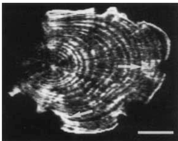
Figure 5. Spin-echo NMR image of a transverse slice through a naturally infected beech ( Fagus sylvatica ) stem with local bark necrosis and staining and incipient decay of the underlying wood. Reaction zones (arrowed) at the margin of these xylem lesions are higher contrast than the healthy wood, suggesting that the water content of reaction zones is elevated in this species also. Scale bar = 10 mm (0.4 in.)
